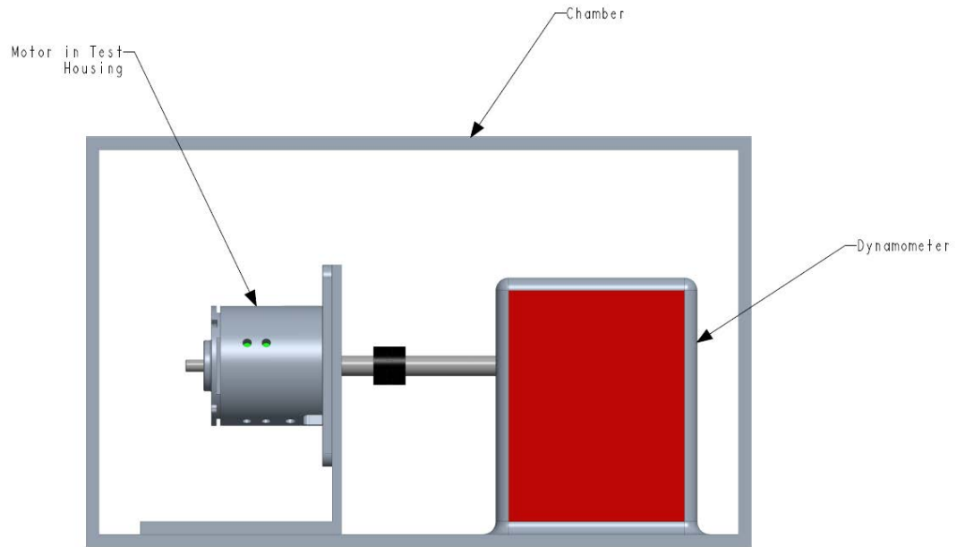
Figure 3: Heat Rise Performance Test Chamber and Fixture Cross Section
